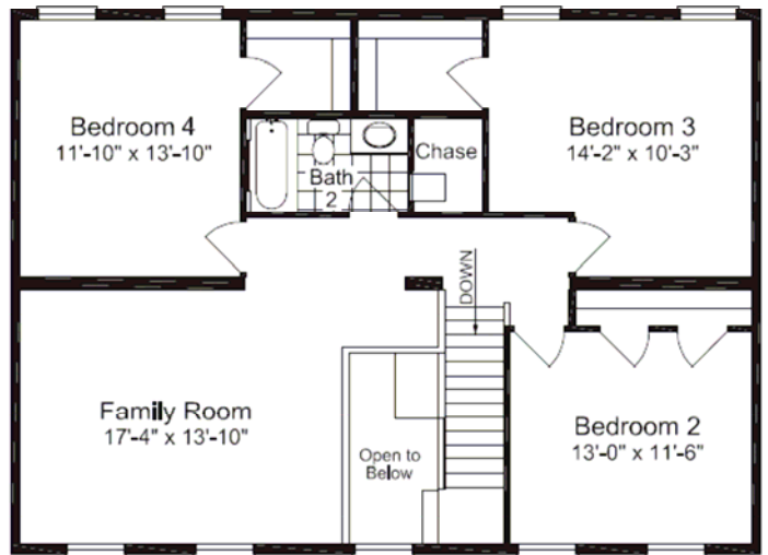
2ND FLOOR
